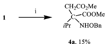
Scheme 2. Alkylation of 1 via radical pathway; i) i\text{PrI} (10 equiv.), \text{Bu}_3\text{SnH} (2.5 equiv.), \text{Et}_3\text{B} (2.5 equiv.), \text{BF}_3\cdot\text{OEt}_2 (2.0 equiv.), \text{ClCH}_2\text{CH}_2\text{Cl} , reflux, 48 h.
